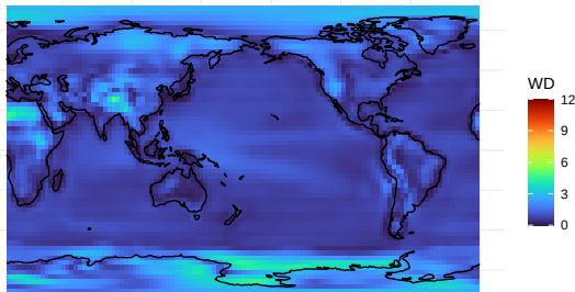
SCWD Map from NCEP Reanalysis to ERA5 Surface Temperature
