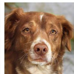
Qwen-7B
