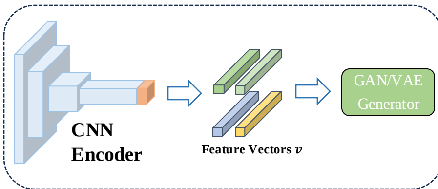
Fingerprinting Model
