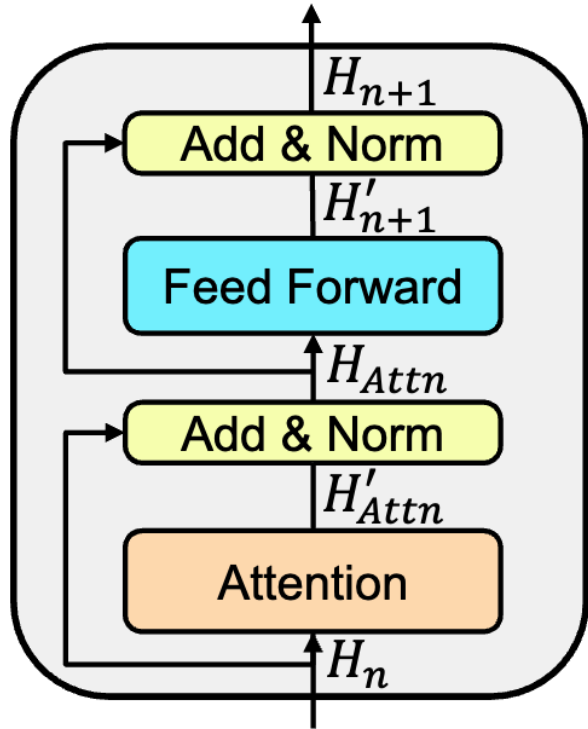
Figure 2: Transformer layer
