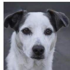
Falcon-40B
